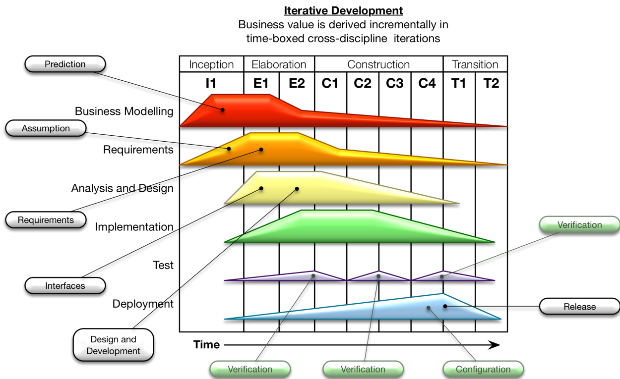
Figure 4: Development lifecycle
